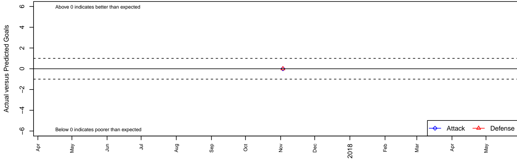
Colorado Rush USSDA B05 Dots are actual minus expected GF (blue circles) and GA (red triangles). Blue line is smoothed change in attack strength. Red is smoothed change in defense strength.
